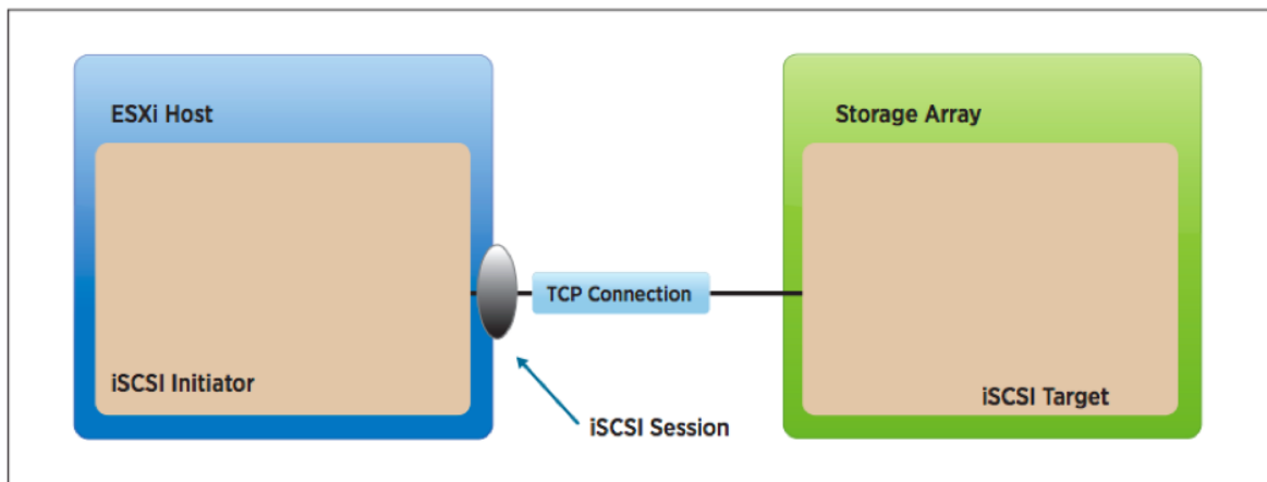
Figure 1 - iSCSI Session
