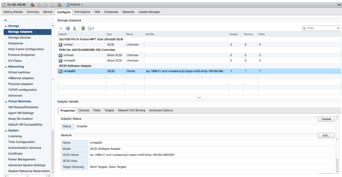
Figure 6 - Enable Software iSCSI Adapter
