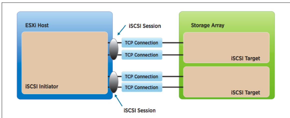
Figure 2 - Multiple connections per session
