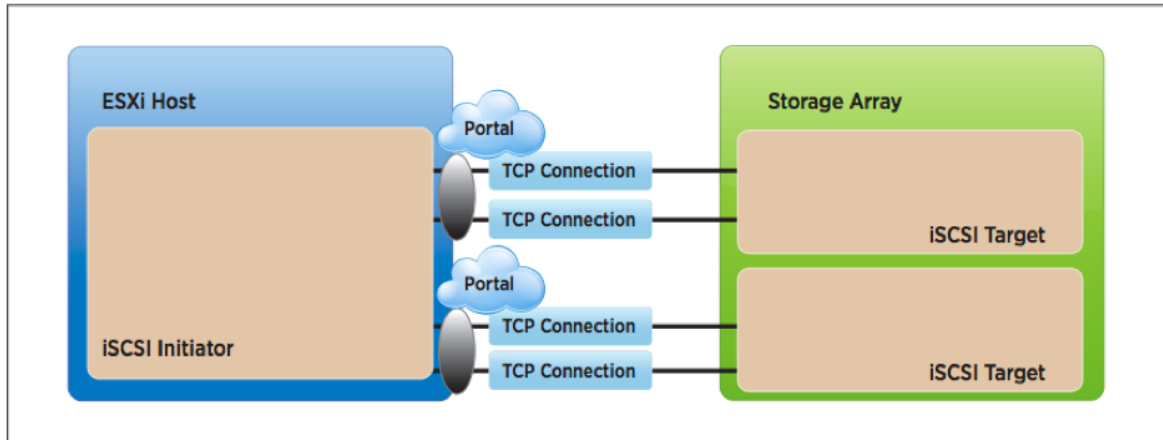
Figure 3 - iSCSI Portals
